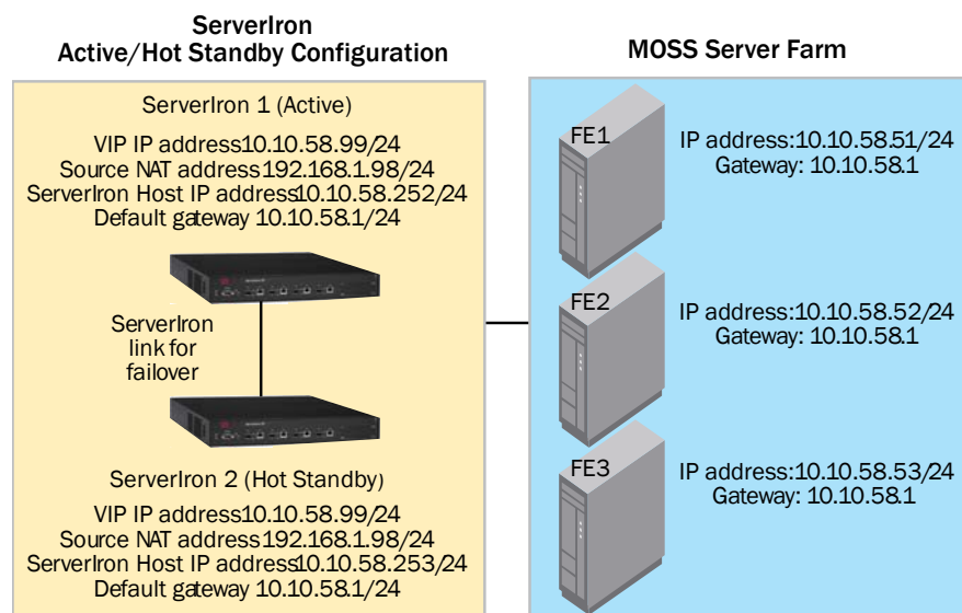
Figure 3. Configuration network topology
