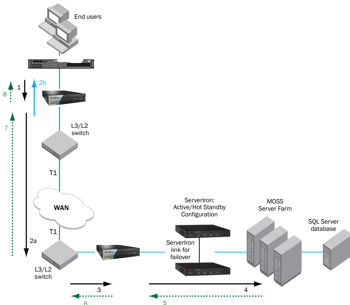
Figure 5. The handshake between a client and the server farm
