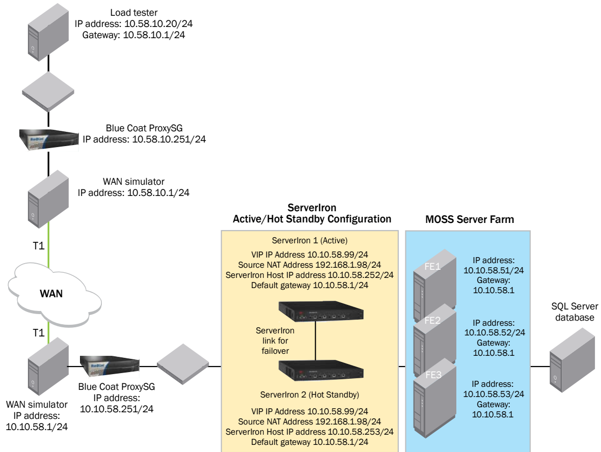
Figure 2. Using an pair of ServerIrons for high availability and Blue Coat ProxySG
