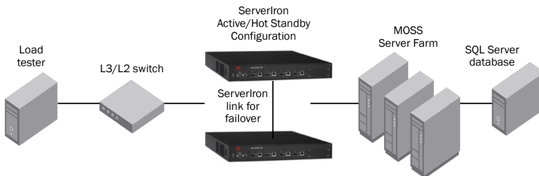
Figure 4. Configuration for SSL offload
