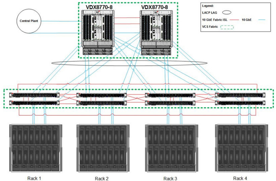
Figure 1: Main Data Center Deployment.
