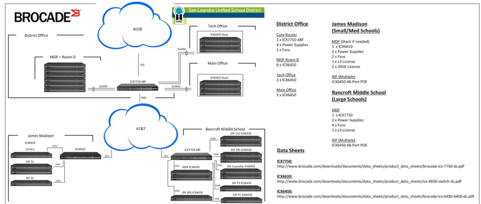
Figure 1. San Leandro School District New End-to-End Network Design
