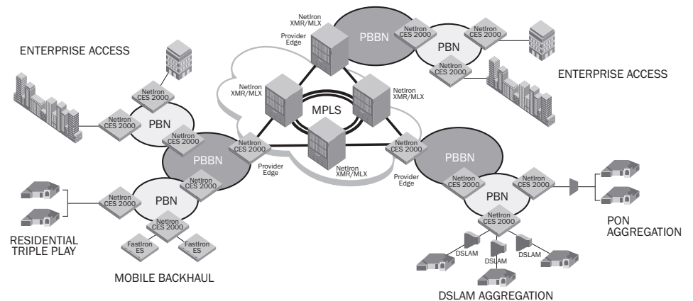
Figure 1: A possible application of using PBB technology on Brocade CES 2000 Series Switches in a large Carrier Ethernet network.
